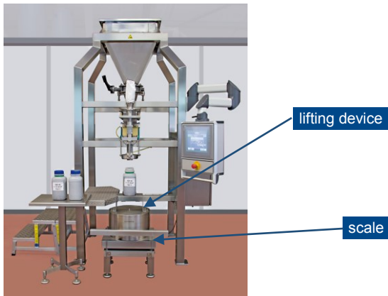
General view with carrying frame, product hopper, dosing channel, scale with mounted lifting lifting device and control system.
